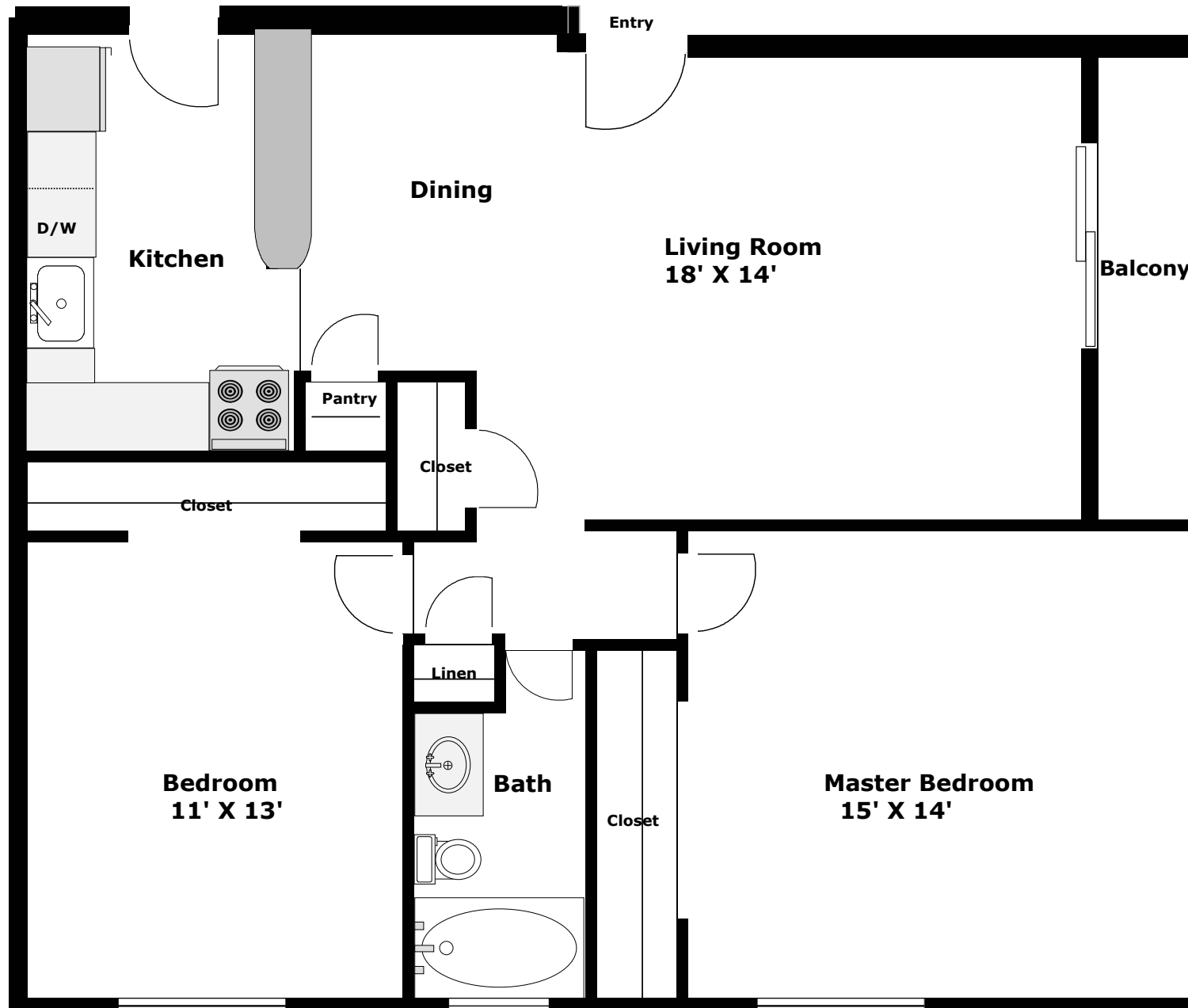
Spanish Trace 2 Bedroom A 980 Sq. Ft.
